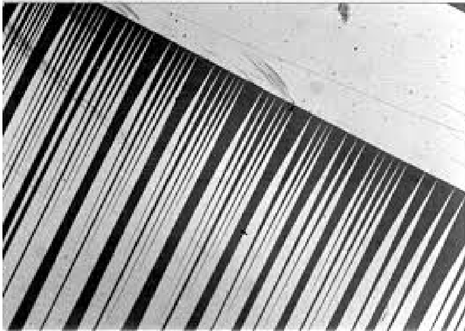
http://www.lasp.cornell.edu/sethna/Tweed/What_Are_Martensites.html
