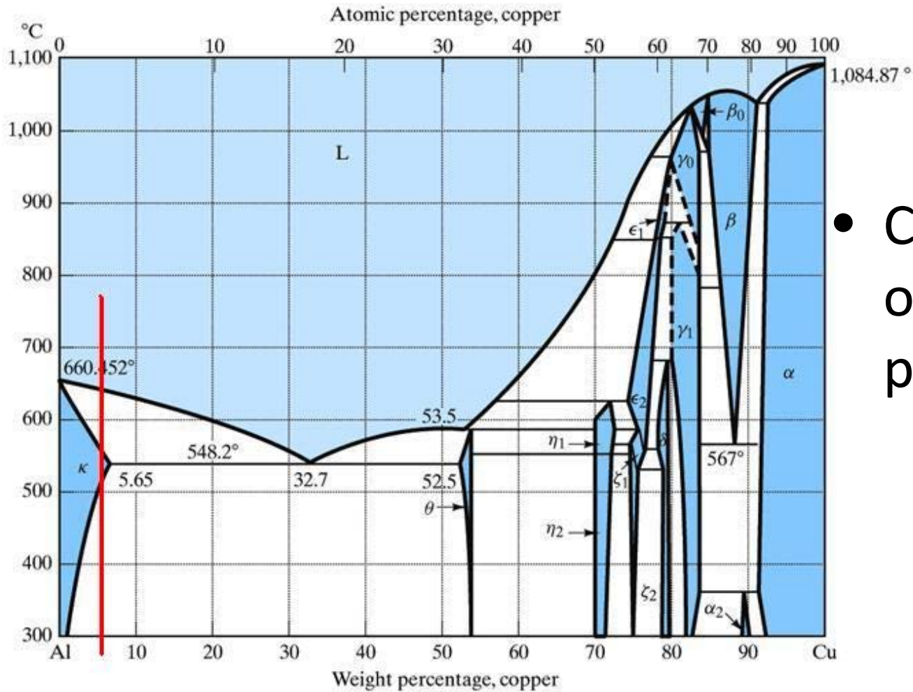
Al-Cu phase diagram
