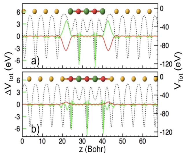
FIG. 4: The total NEGF-LSDA spin down potential ( V_{Tot} = V_{Tot}^{LSDA} ) is shown as a dotted black line, with its axis given on the right hand side of the figure (the vacuum level is set at 0 eV). The bulk LSDA SEP interface error is shown in green ( \Delta V_{Tot} = V_{Tot}^{SEP} - V_{Tot}^{LSDA} ) and the interface spherical SEP correction to the error is shown in red (both potentials are read off the left axis). Subfigure a) displays the system potential as a linear cut in the z -direction through the Mg atom at the Fe/MgO interface. Subfigure b) displays the system potential as a linear cut in the z -direction through the FeO bond at the Fe/MgO interface. An atomistic cartoon is shown to scale above each potential plot, where a dip in the total potential corresponds to an atomic nuclear position – Fe atoms are gold, O atoms are red, and Mg atoms are green. Up spin results are nearly identical. The SEP MgO band gap corrections (see Figs. 1 and 2) are not included in this comparison.
