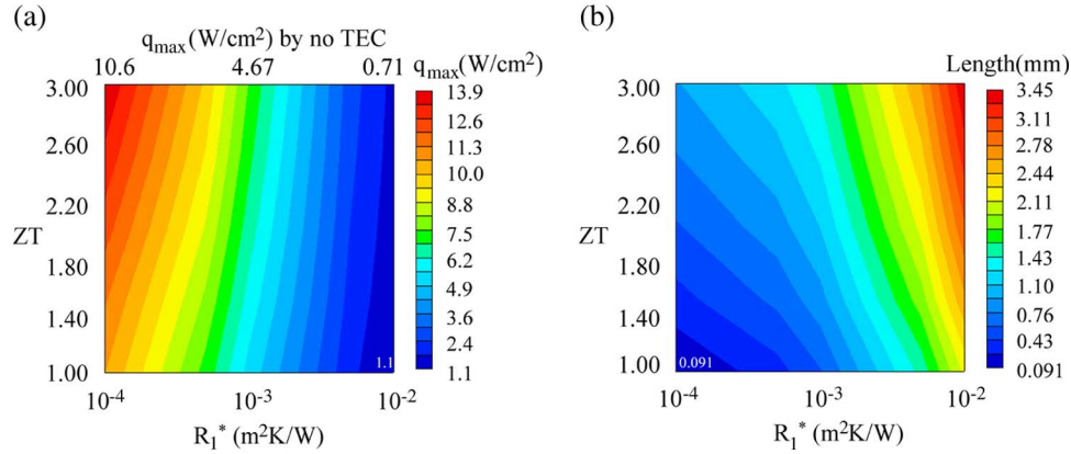
Fig. 8. Effect on R_1^* and ZT on q_{\max} (W/cm 2 ) at T_{\text{chip}} = 100^\circ\text{C} and optimum leg length is shown. (a) Contour plot of q_{\max} as a function of R_1^* and ZT . (b) Contour plot of optimized L for each q_{\max} as a function of R_1^* and ZT . R_2^* = 6.05 \times 10^{-4} m 2 K/W (current technology value) is assumed.
