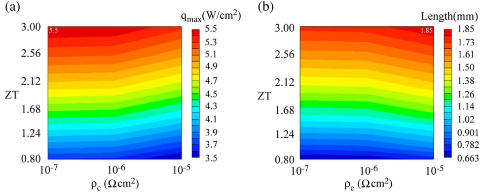
Fig. 9. Effect of \rho_c and ZT on q_{\max} (W/cm²) at T_{\text{chip}} = 100^\circ\text{C} and optimum length is shown. (a) Contour plot of q_{\max} as a function of \rho_c and ZT . (b) Contour plot of optimized L for each q_{\max} as a function of \rho_c and ZT . R_1^* = 1.73 \times 10^{-3} \text{ m}^2\text{K/W} and R_2^* = 6.05 \times 10^{-4} \text{ m}^2\text{K/W} (current technology values) are assumed for the calculation.
