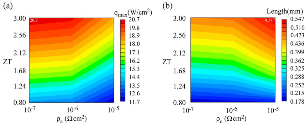
Fig. 10. Effect of \rho_c and ZT on q_{\max} (W/cm²) at T_{\text{chip}} = 100^\circ\text{C} and optimum length is shown when R_1^* and R_2^* are improved by a factor of 3.75 compared with the current technology values. (a) Contour plot of q_{\max} as a function of \rho_c and ZT . (b) Contour plot of optimized L for each q_{\max} as a function of \rho_c and ZT . R_1^* = 4.61 \times 10^{-3} \text{ m}^2\text{K/W} and R_2^* = 1.61 \times 10^{-4} \text{ m}^2\text{K/W} are assumed.
