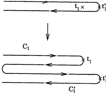
FIG. 2: Deformation of contour C
